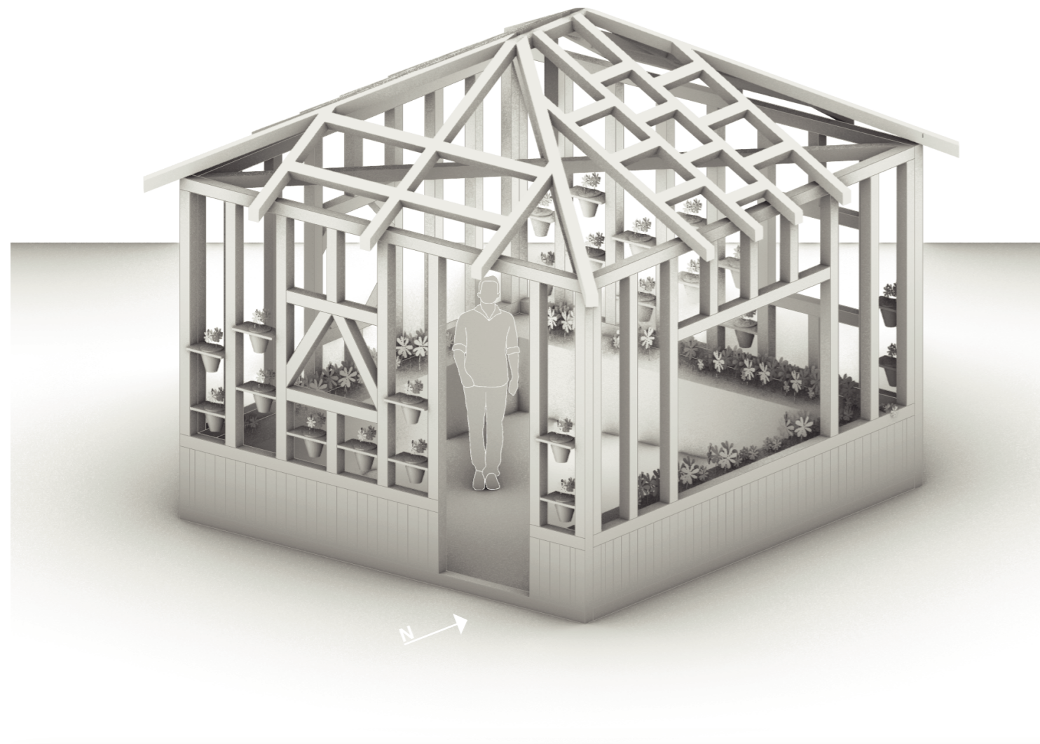
Isometrical view
