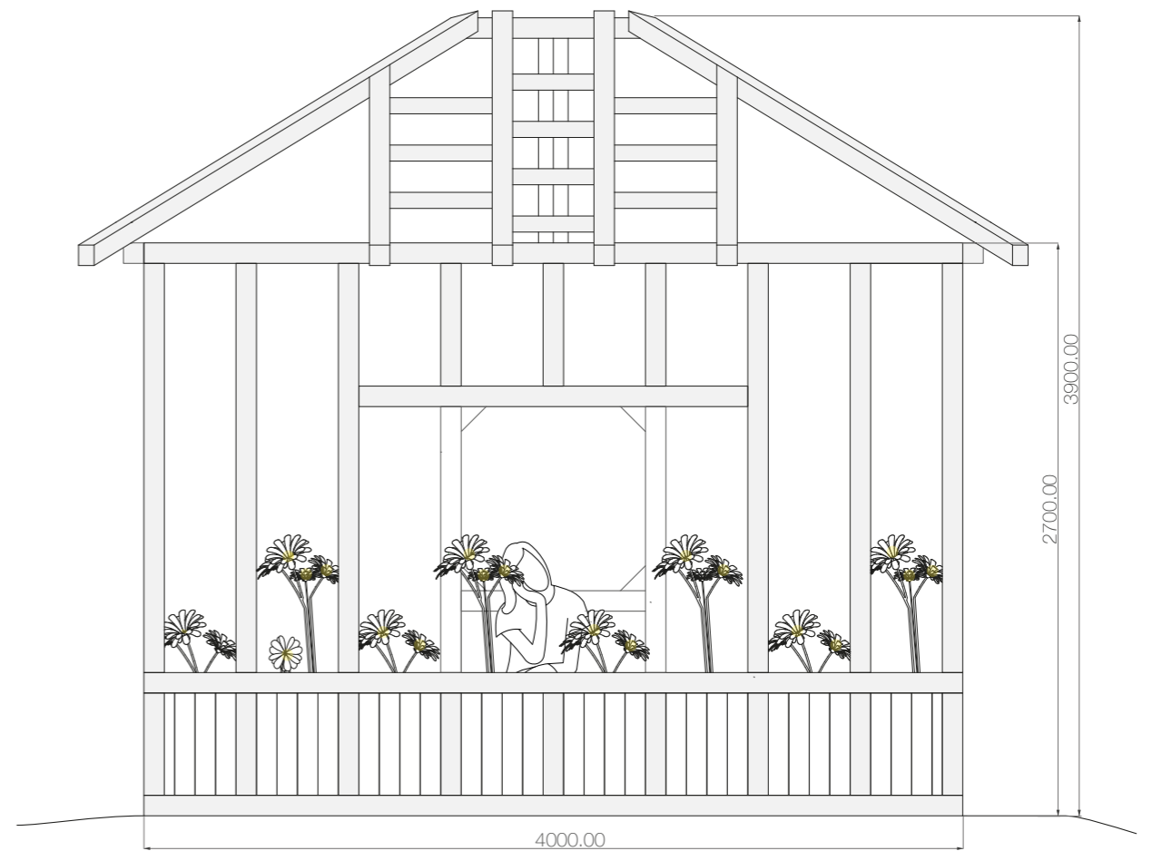
East elevation
