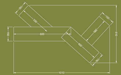
RHIZOME in SHEET of EXPANDED METAL
