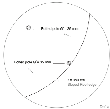
Det' a Roof plan
