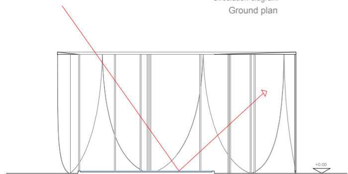
Direct sun light path / Reflective plate Sec a'a
